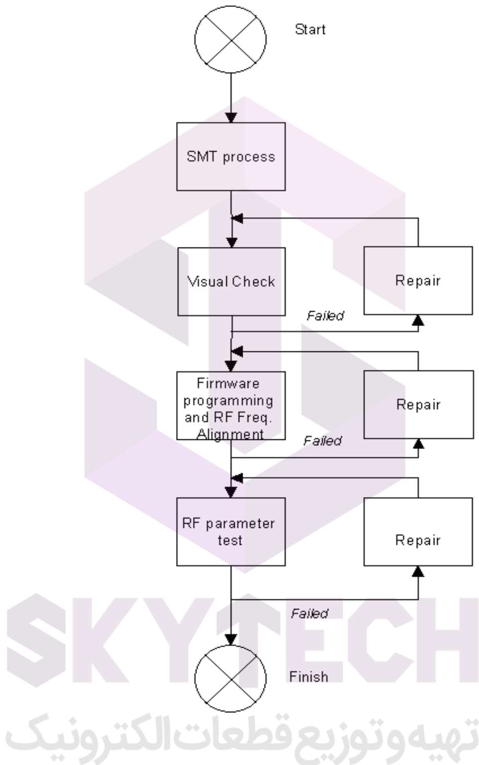
Fig 3 Assemble/Alignment/Testing Flow Chart
